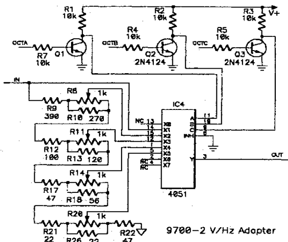
Fig 6. The V/Hz Adapter circuit is a voltage divider with taps at octave ratios of 1, 1/2, 1/4, 1/8 and 1/16
