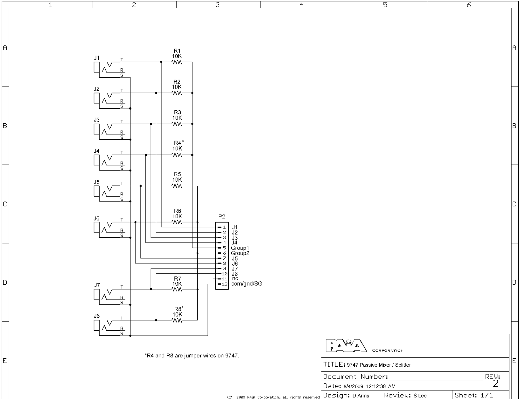
Fig.2 Passive Mixer-Splitter Schematic
