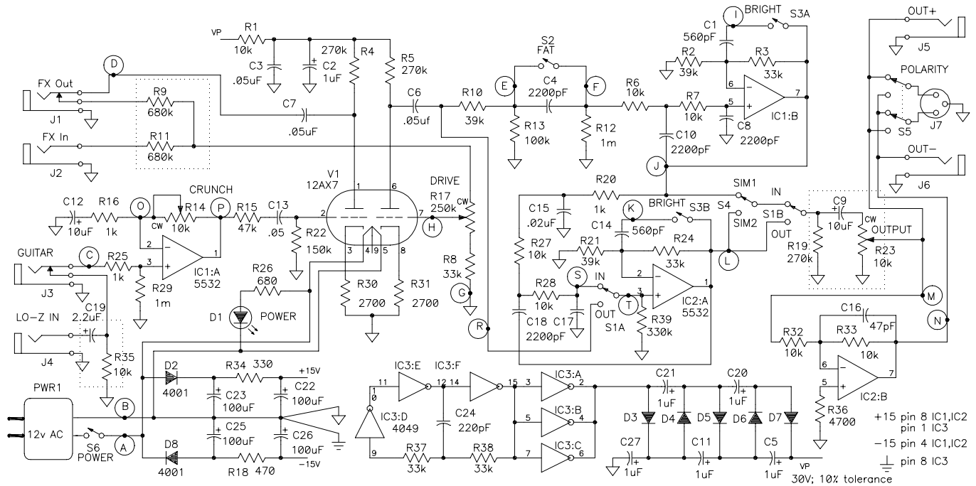
Stak-in-a-Box Schematic (c) 2000 PAiA all rights reserved fair use copy with this notice only contact: info@paia.com
